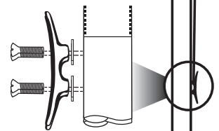
Attach rope cleat with screws and washers
