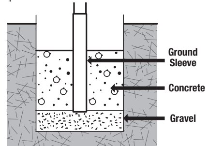
Fill with concrete 6" from the top of the ground sleeve. When concrete sets, fill around pole with ground cover.
